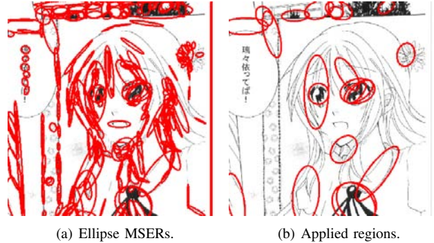
Figure 2. Examples of ellipse MSERs and candidate regions.
